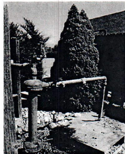
Figure 1: The wellhead on your property will typically include a pipe leading to your pressure tank.
